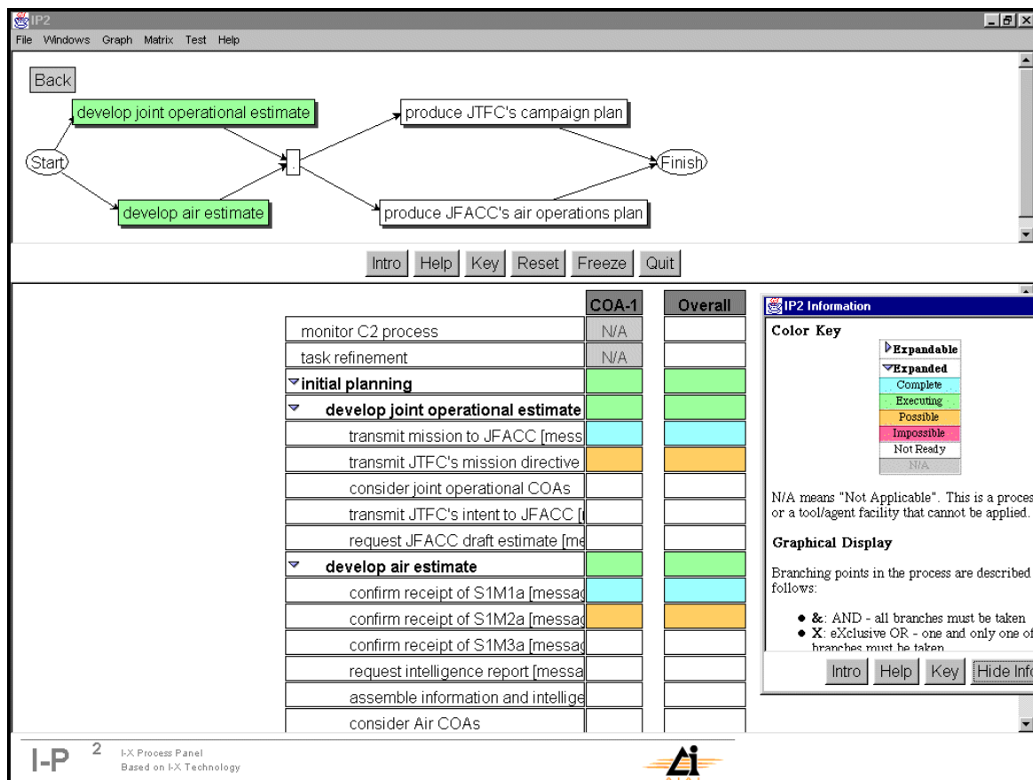
Figure 5 - The Process Panel
