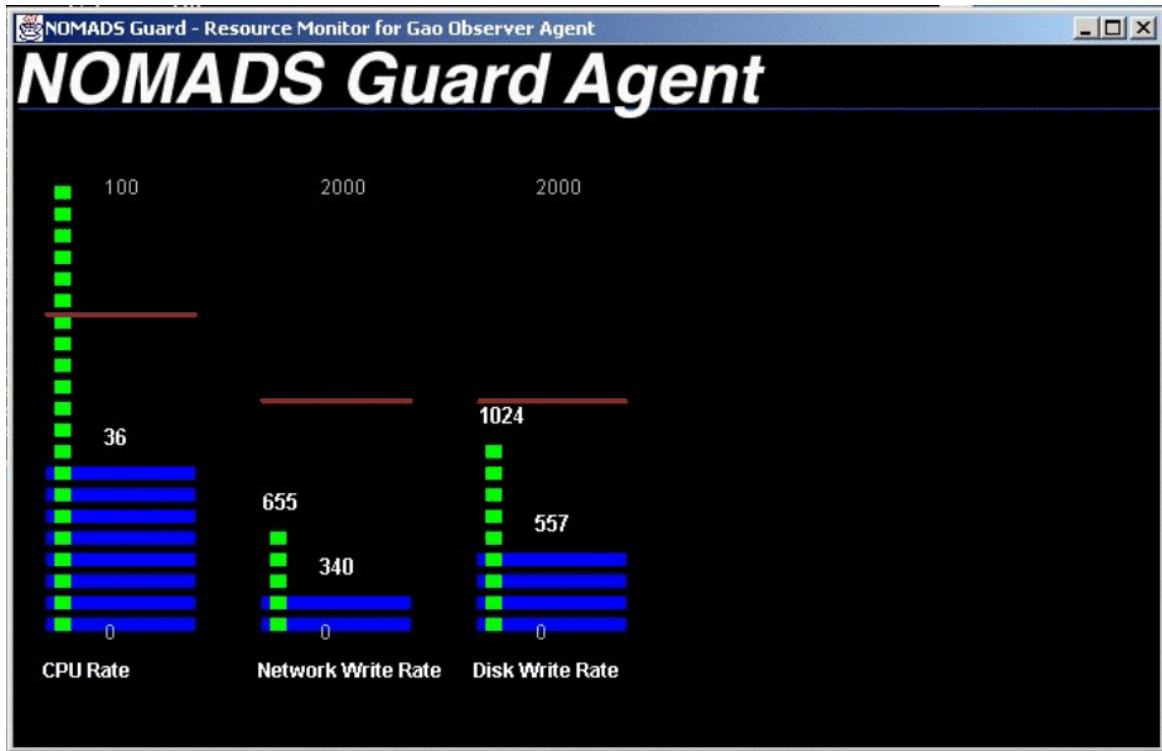
Figure 7 - The NOMADS Guard Display
